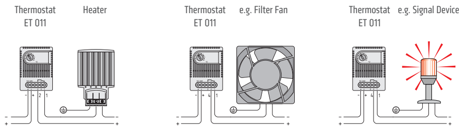
Wiring examples
