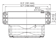
Screw mount
